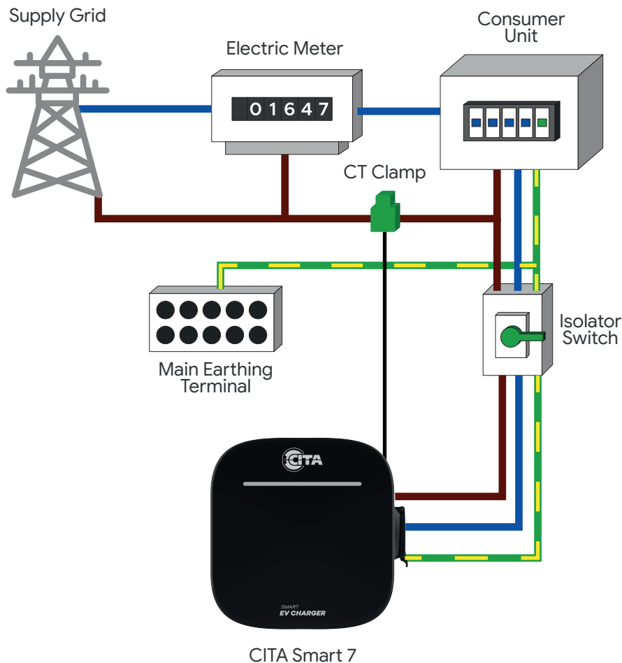
CT Clamp Installation schematic diagram
